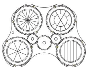
Prism 2: 4 different prisms, 6-Facet linear prism/6-Facet circular prism/8-Facet circular prism/16-Facet circular prism with variable speed and direction Prism indexing
