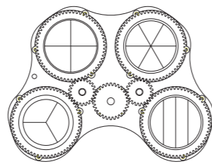
Prism 1: Prism 1: 4 different prisms, 4-Facet linear prism/3-Facet circular prism/4-Facet circular prism/6-Facet circular prism with variable speed and direction
